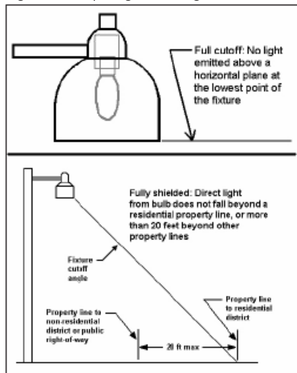
Figure 7.7: Proper Light Shielding
